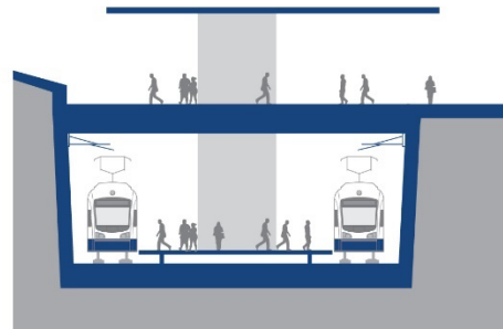
Retained-Cut Center-Platform Station with Lid
