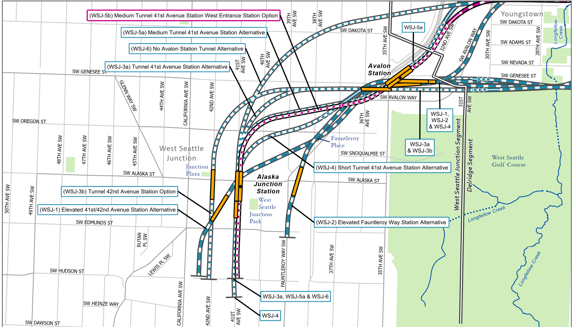
FIGURE 2-34 West Seattle Junction Segment Alternatives West Seattle Junction Segment
