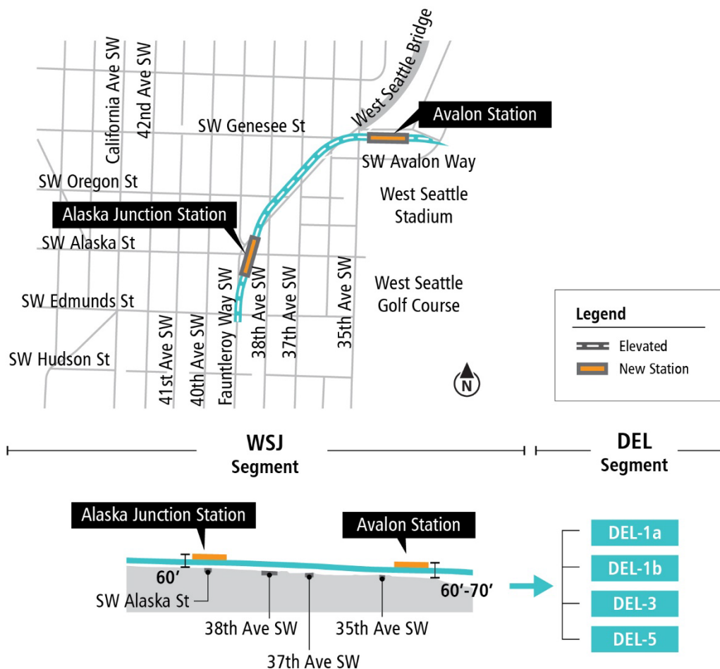
Figure 2-37. Plan and Profile for Elevated Fauntleroy Way Station Alternative (WSJ-2)
