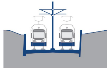
Retained-Cut Guideway
