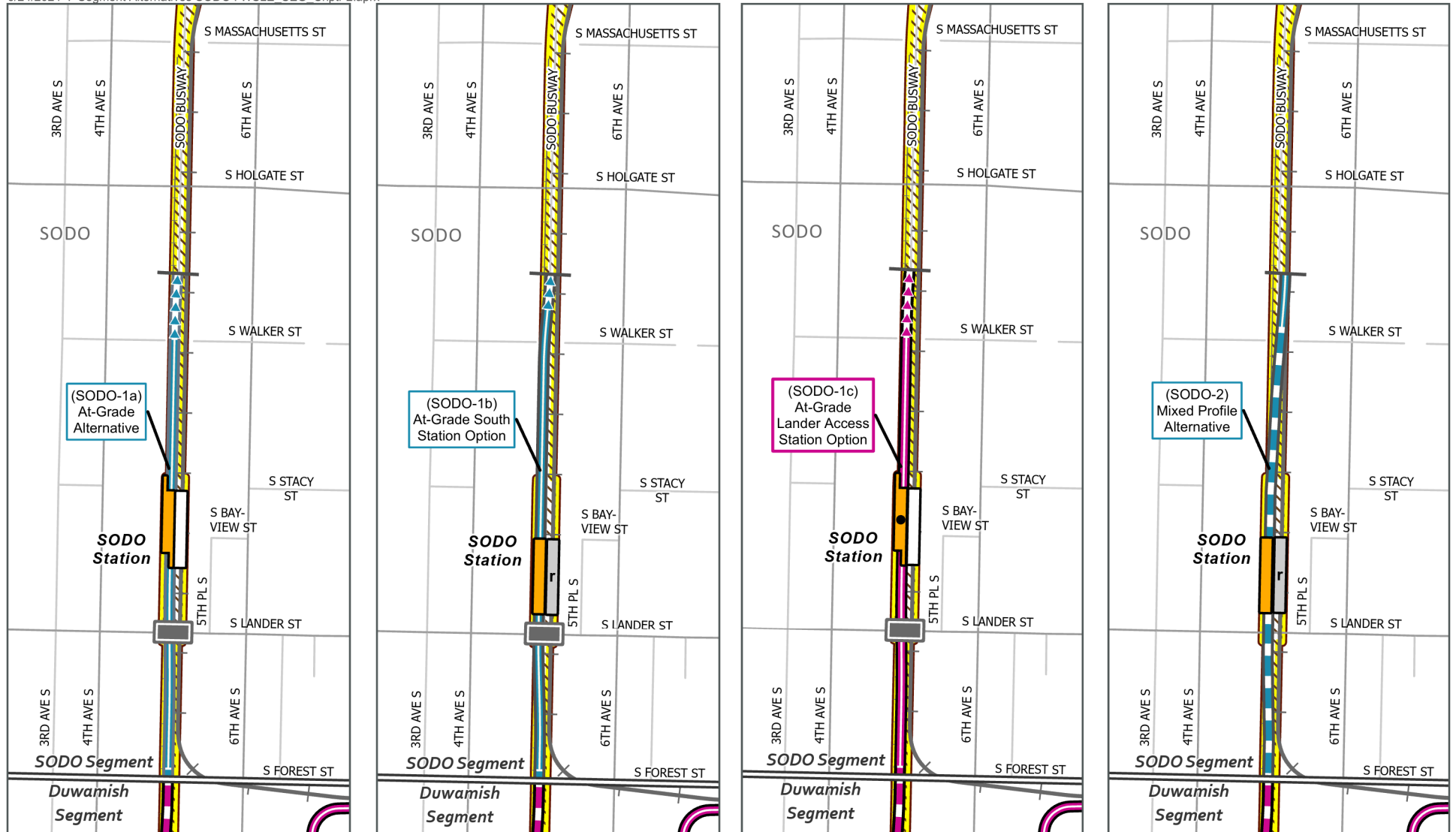
FIGURE 2-14 SODO Segment Alternatives SODO Segment West Seattle Link Extension
