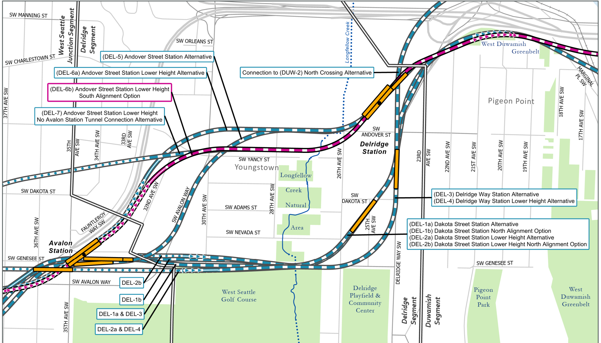
FIGURE 2-23 Delridge Segment Alternatives Delridge Segment
